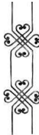
ED67 Sect: 12x6 mm H: 900 mm L: 250 mm
