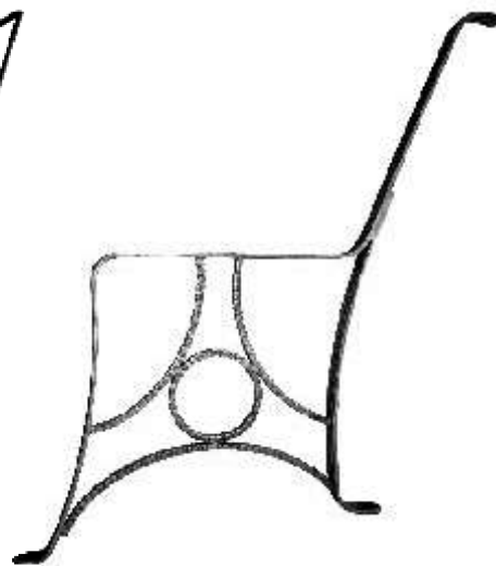
PBC982 H1: 940 mm H2: 500 mm L: 470 mm Sect: 40x4 mm
