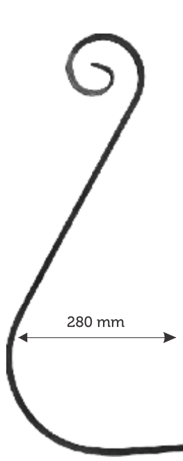
EC008 Sect: 12x12 mm H: 800 mm L: 280 mm Amprentat
