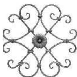
PN016.26 Sect: 16x6 mm H: 480 mm L: 410 mm Amprentat
