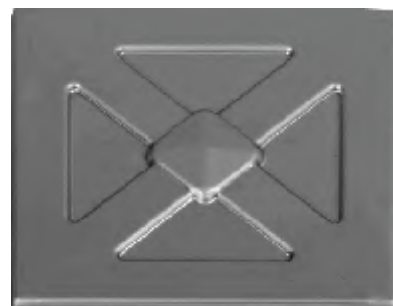
DC042 H: 250mm L: 250mm Gr.: 1,2mm
