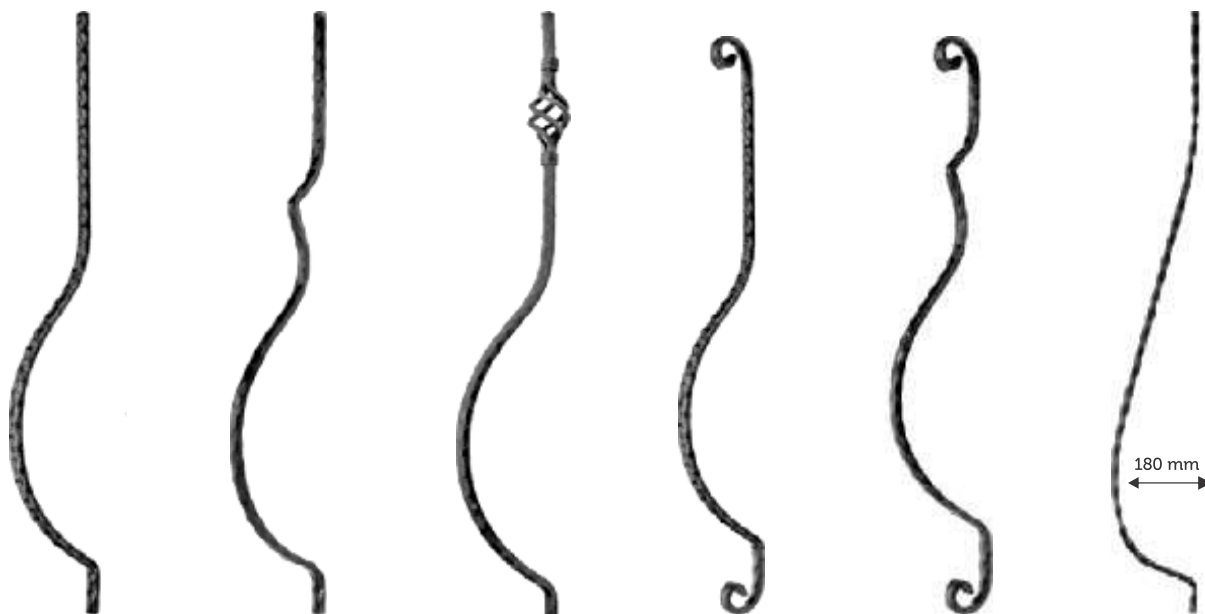
EC01 Sect: 12x12 mm H: 900 mm L: 150 mm
