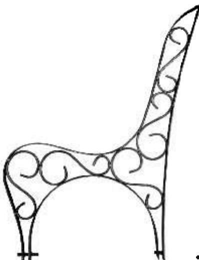
PBC981 H1: 1000 mm H2: 640 mm L: 470 mm Sect: 40x4 mm
